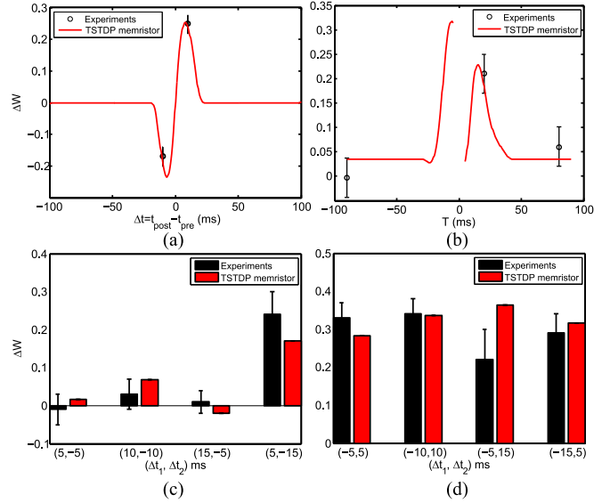
Fig. 7. (a) Proposed triplet-based STDP memristive synapse reproduces the STDP learning window. (b) The proposed TSTD device predicts similar weight changes to the data presented in [15] for quadruplet protocol. Note that there is no experimental data available around 0 ms. (c)–(d) The proposed synapse, correctly distinguishes between (c) pre-post-pre triplet case, and (d) post-pre-post triplet case.
