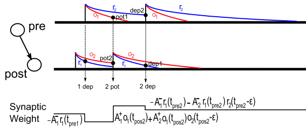
Fig. 3. Synaptic weight changes, at the time of each spike, as a function of the timing difference between pre- and post-synaptic spikes, their temporal order, and their synaptic amplitude parameters, i.e., A_1^+ , A_1^- , A_2^+ and A_2^- .
